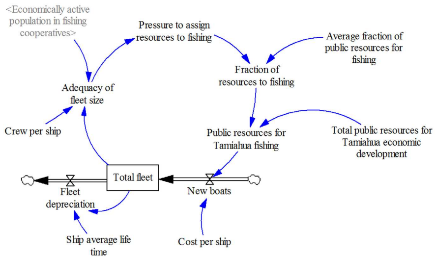
Figure 4. Fleet growth
