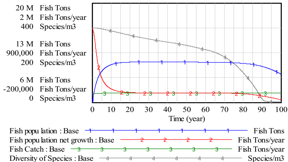
Figure 7. Fish population
