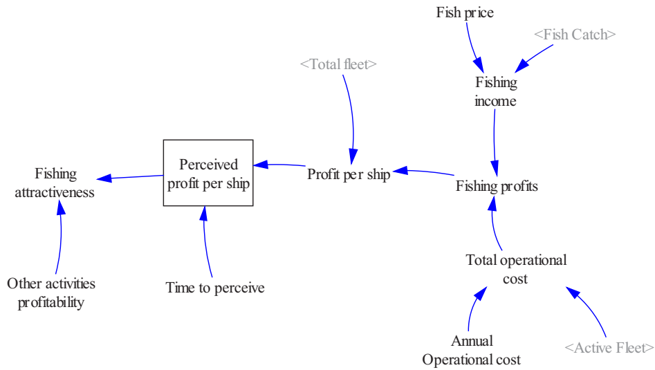
Figure 3. Fishing attractiveness
